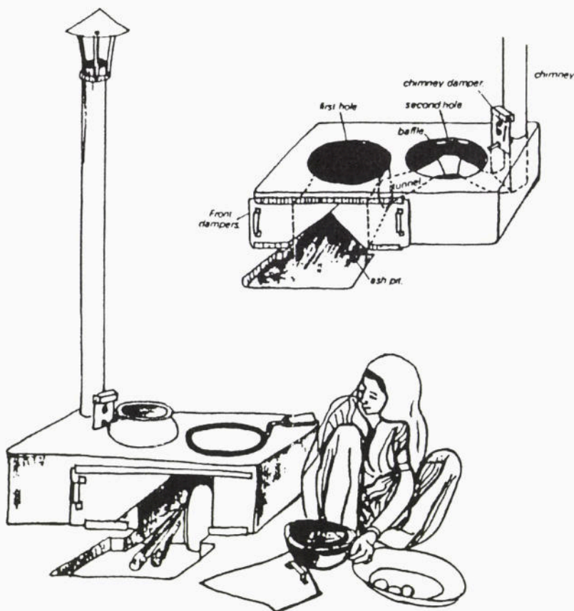
Taken from: CHULHA MISTRI TRAINING MANUAL by Madhu Sarin, India
